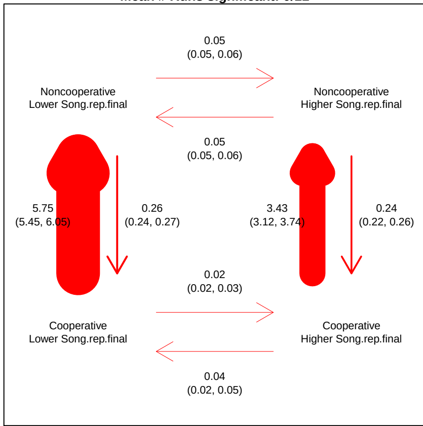
Thresholds \geq 1 - < 8.5 (23) Mean # Runs significant: 0/11
