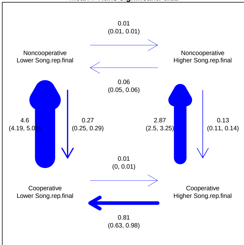
Thresholds \geq 34 - < 1450 (23) Mean # Runs significant: 0/11
