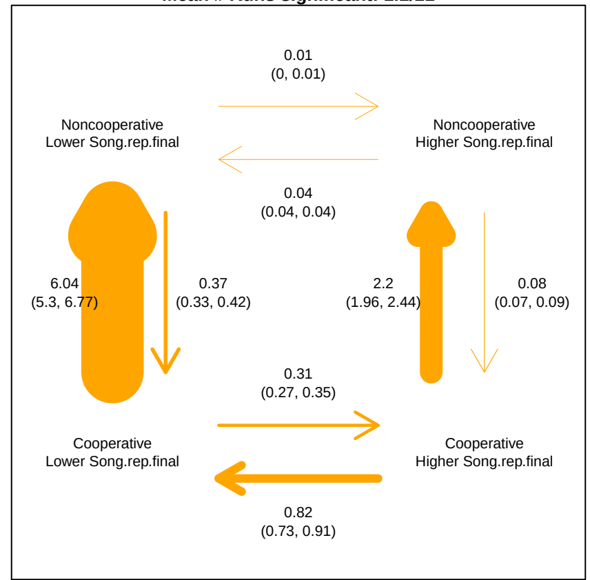
Thresholds \geq 8.5 - < 34 (24) Mean # Runs significant: 1.1/11
